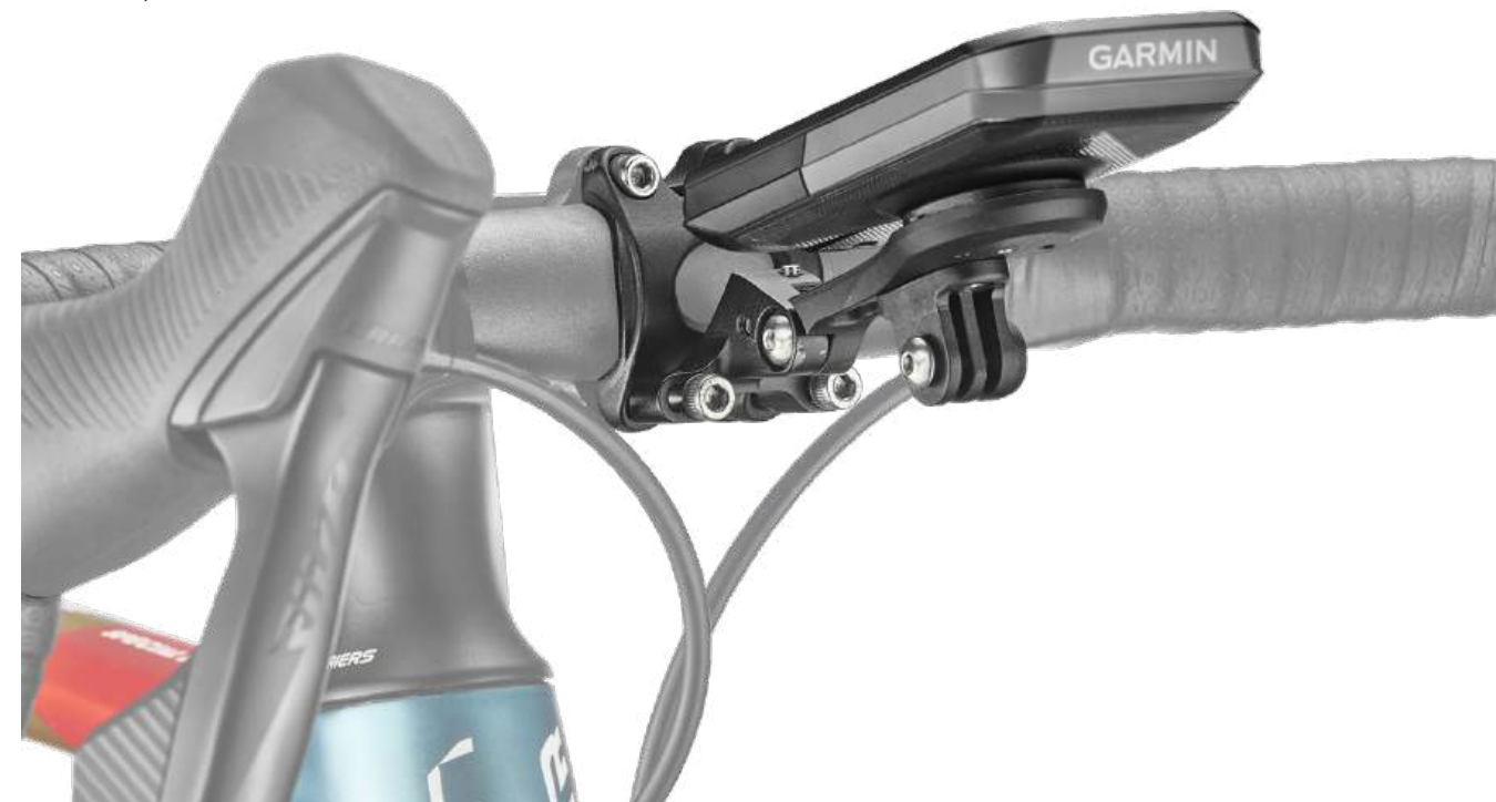
Bracket fatigue test method: Impact 150kg/f at the stem/handle-bar. load of 1,000 grams at the extension arm and run for 100,000 times.
