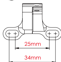
Fit stem screw distanc
